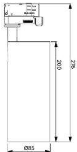
LEDspot3C-C-P 25W
