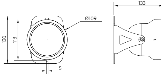
560006001000 - LEDSmart-Sensor IP65-Module
