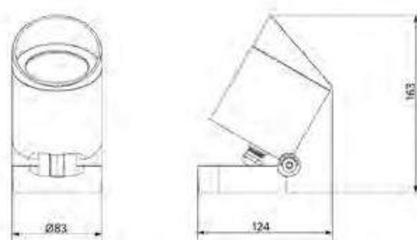
LEDspotProjector-E Rd82
