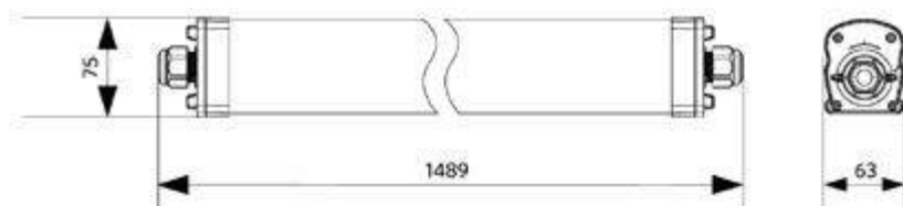
LEDWaterproof-P4 L1489
