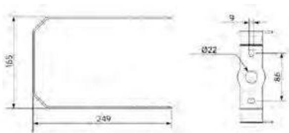
LEDHighbay-E2 Bracket
