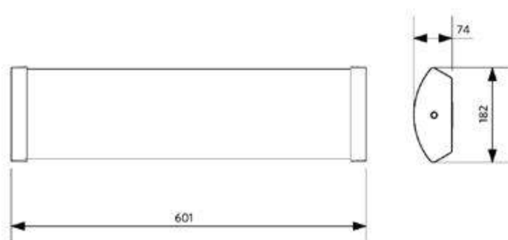
LEDLinear-E CL12
