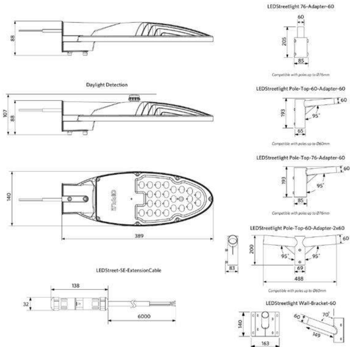
LEDStreetlight-E2
