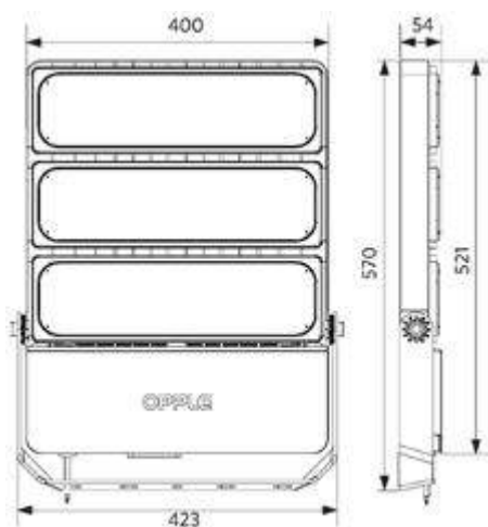
LEDFloodMo-P Re570
