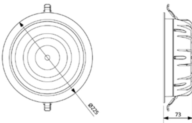
LEDDownlightRc-P-HG R200
