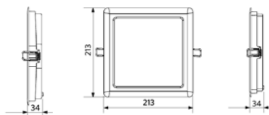
LEDDownlightRc-SI-E Sq200
