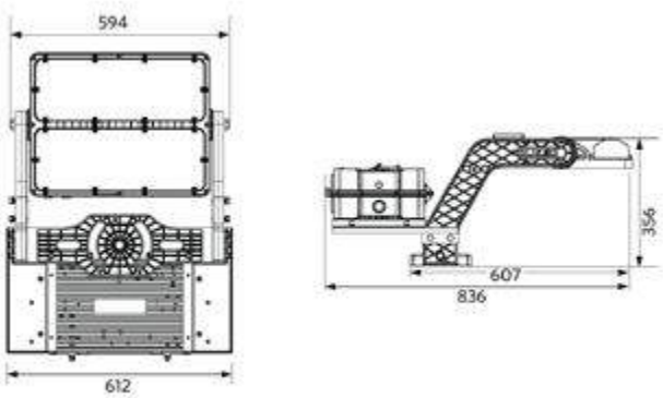
LEDfloodOly-P Re600-800W
