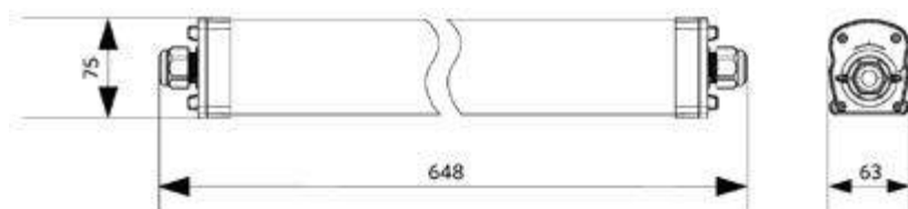
LEDWaterproof-P4 L1208
