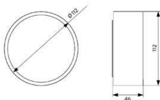
LEDCeilingLu-E Rd112
