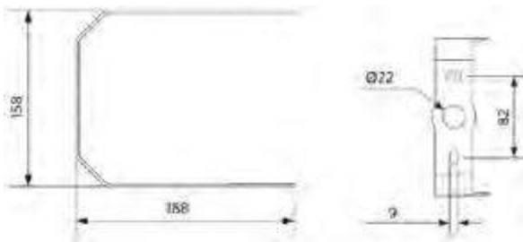
LEDHighbay-P5 Bracket-D330
