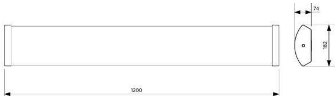
LEDLinear-E CL15
