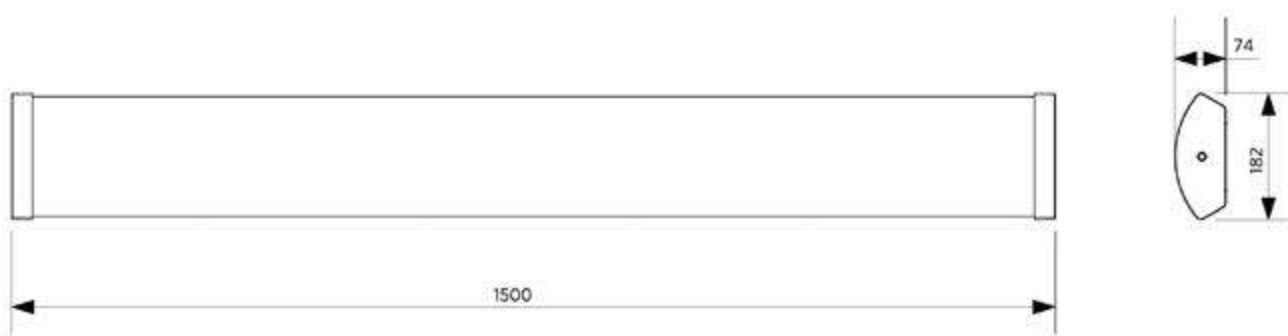
LEDLinear-E CL15
