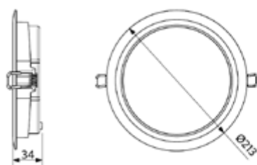
LEDDownlightRc-SI-E Rd200
