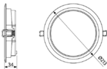
LEDDownlightRc-SI-E Rd200
