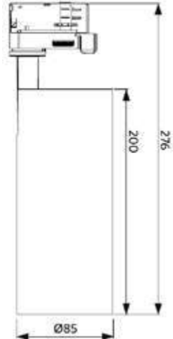
LEDspot3C-C-P 25W
