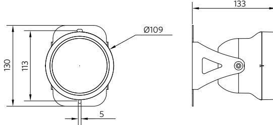
560006001000 - LEDSmart-Sensor IP65-Module
