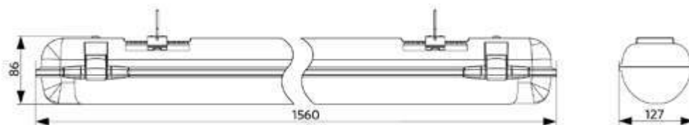
LEDWaterproof-CLA-E L1550
